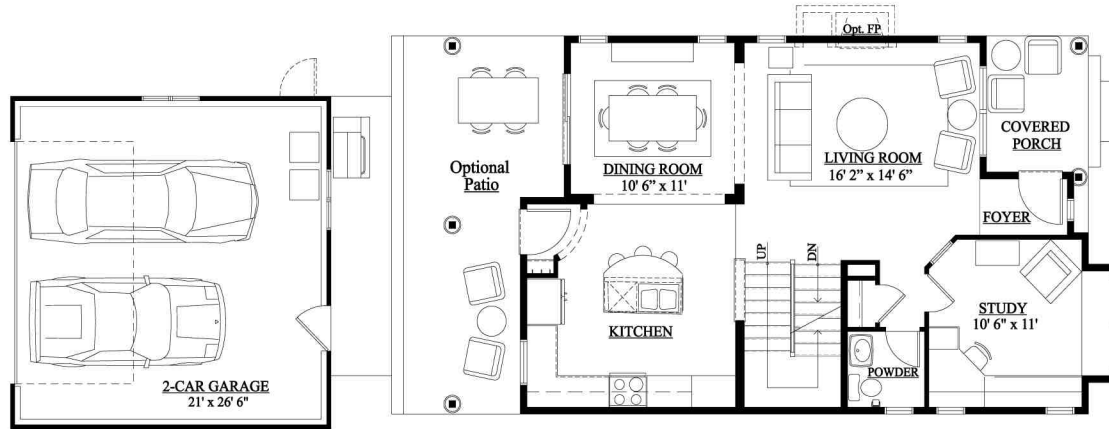
MONTVIEW > FEDERAL MAIN LEVEL – 876 SQ. FT.
