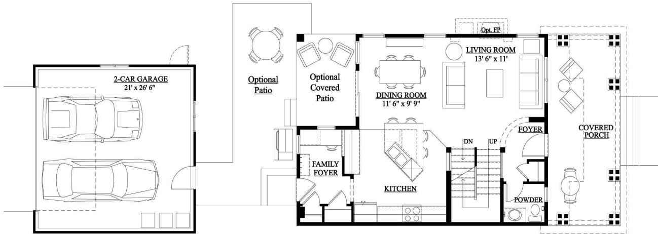
LARIMER > PRAIRIE MAIN LEVEL – 754 SQ. FT.
