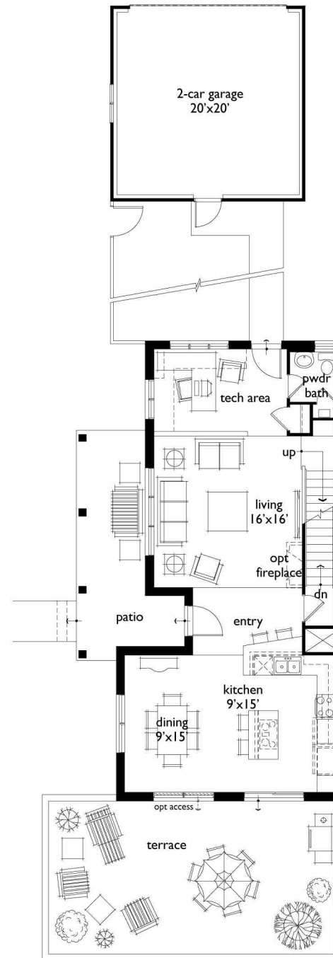
Main Level 947 sf
