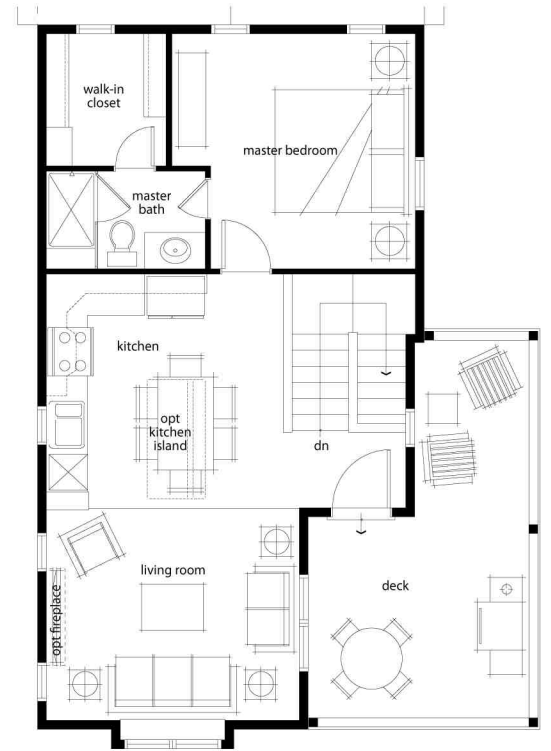
Upper Level-Elevation 2
