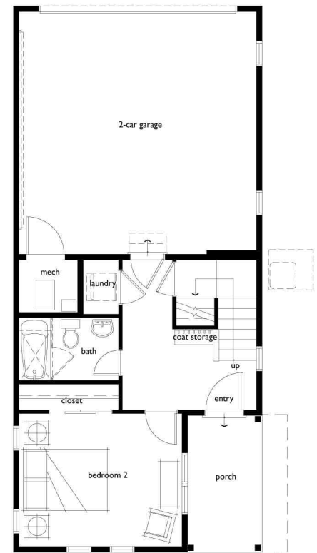
Lower Level-Elevation 1
