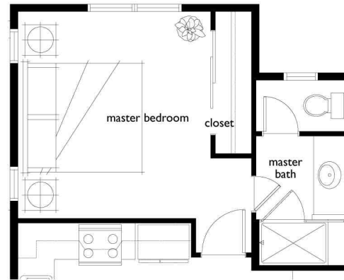
Upper Level-Elevation 1 Optional Master Bath Shower with Bench
