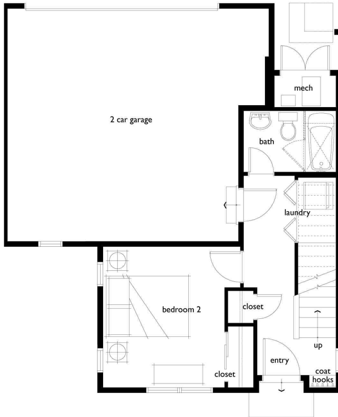
Lower Level-Elevation 1
