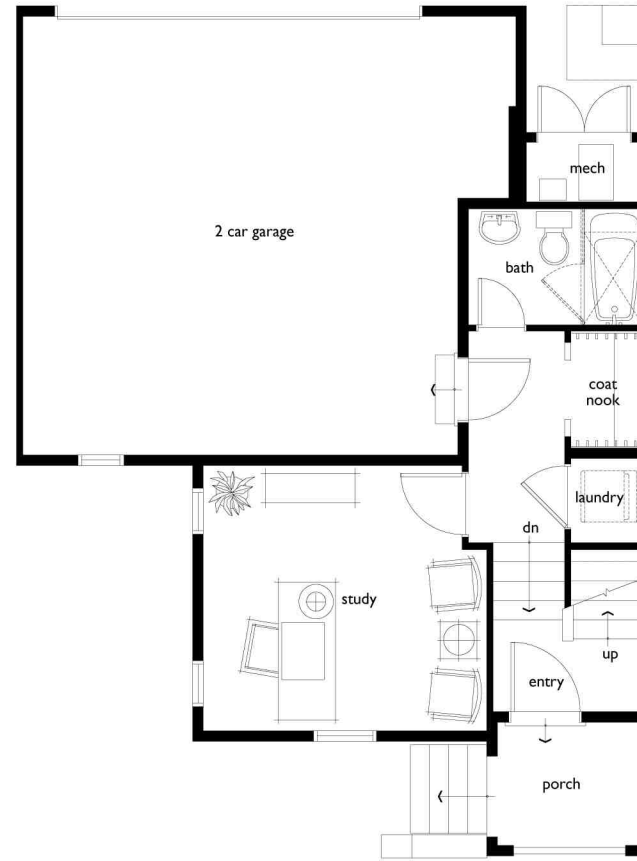
Lower Level-Elevation 1 Optional Study in Lieu of Bedroom
