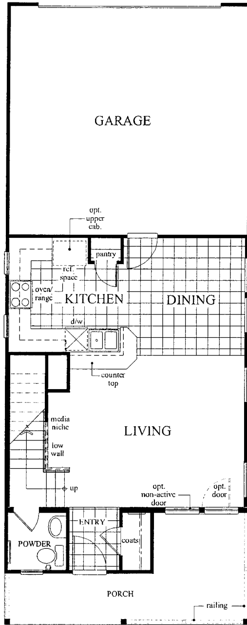
FLOOR PLAN
