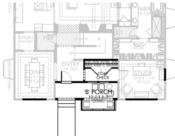
MAIN LEVEL OPTIONAL 'B' ELEVATION PLAN
