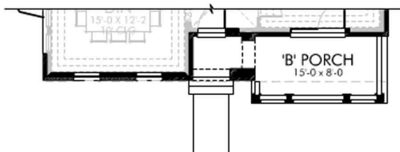
MAIN LEVEL OPTIONAL 'B' ELEVATION PLAN
